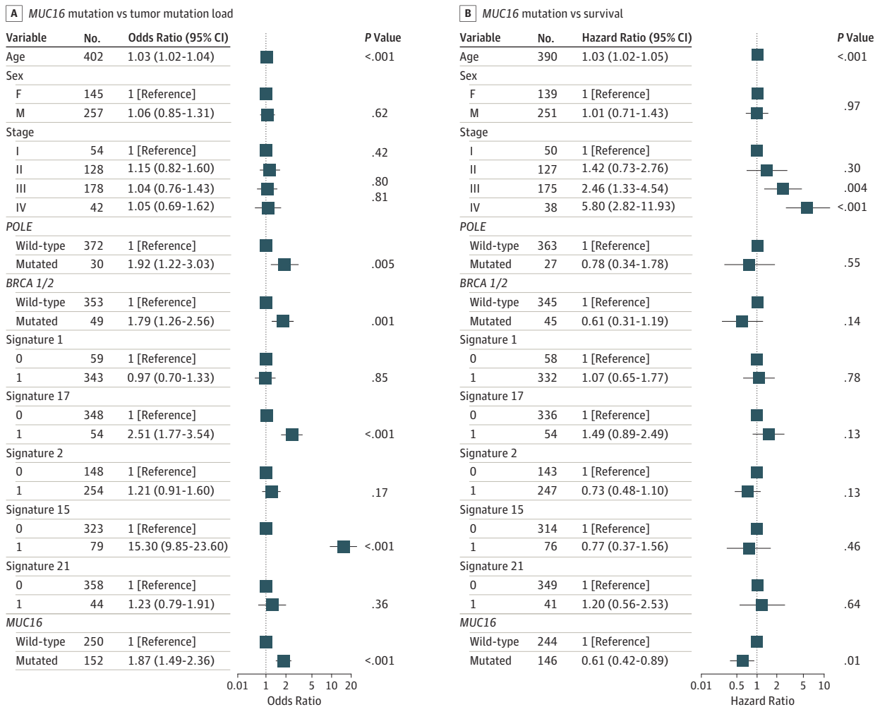
Figure 3. Association of MUC16 Mutation With Higher Tumor Mutation Load and Survival Outcome in The Cancer Genome Atlas Cohort of Gastric Cancer Samples
