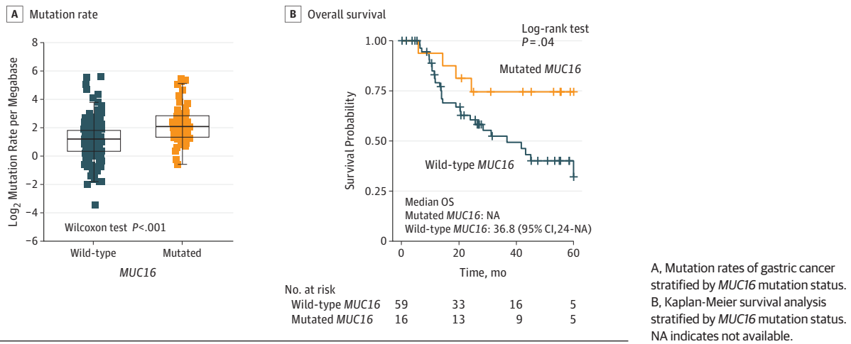
Figure 5. Association of MUC16 Mutation With Tumor Mutation Load and Survival Outcome in the Asian Cohort
