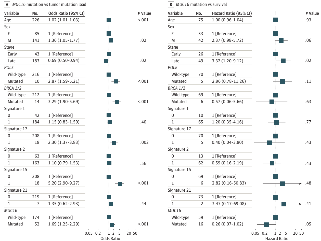
Figure 5. Association of MUC16 Mutation With Tumor Mutation Load and Survival Outcome in the Asian Cohort
