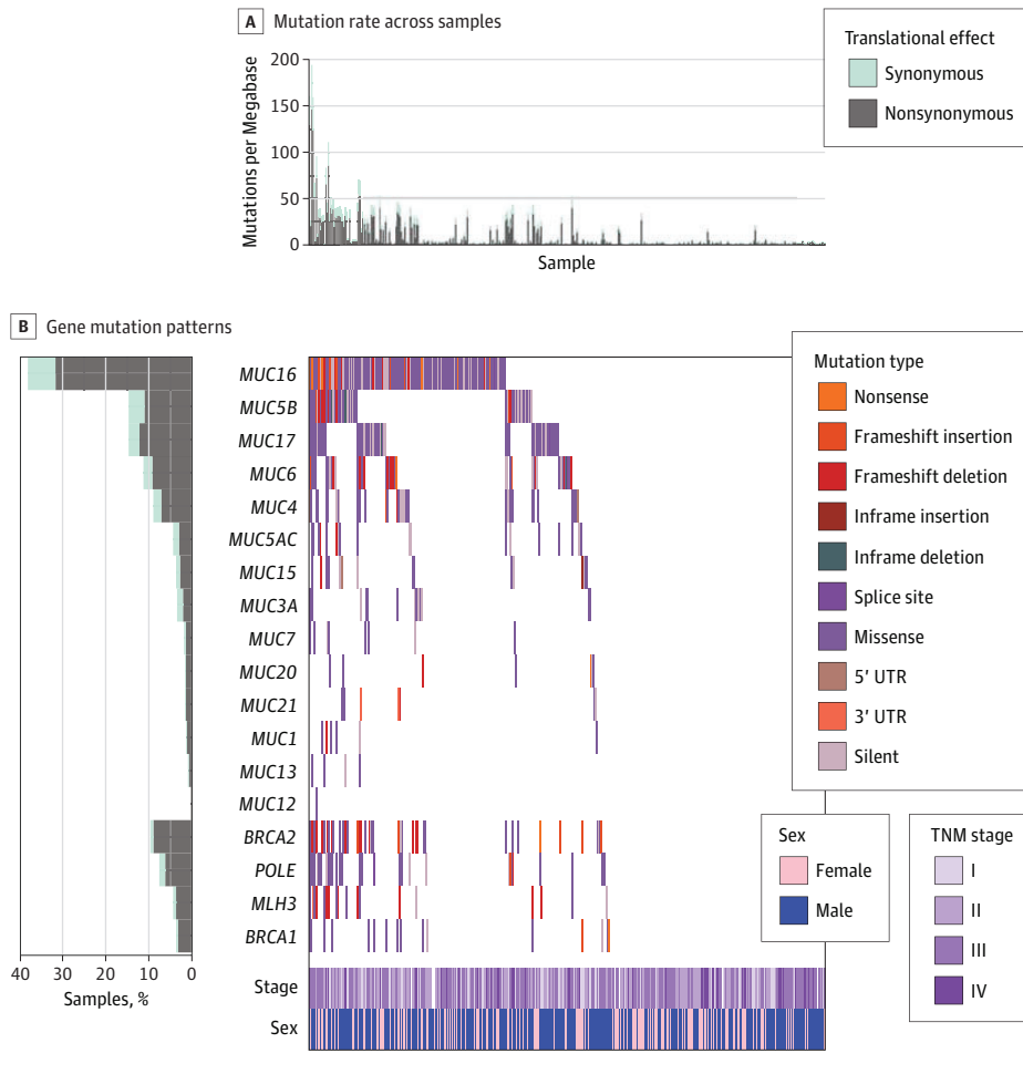
Figure 2. Association of MUC16 Mutation With Tumor Mutation Load and Prognosis in The Cancer Genome Atlas Cohort
