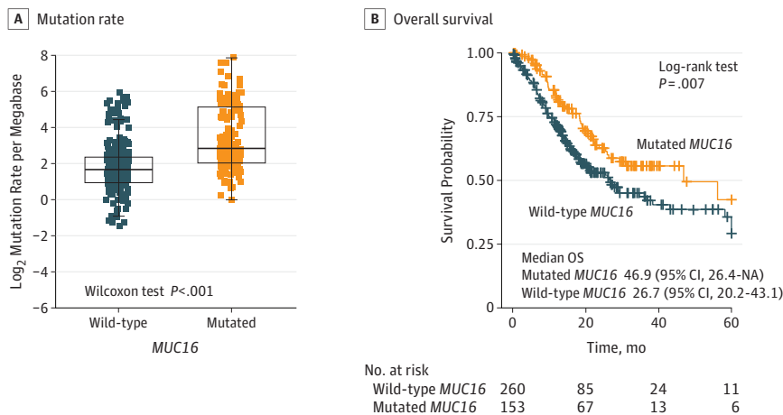
Figure 2. Association of MUC16 Mutation With Tumor Mutation Load and Prognosis in The Cancer Genome Atlas Cohort
